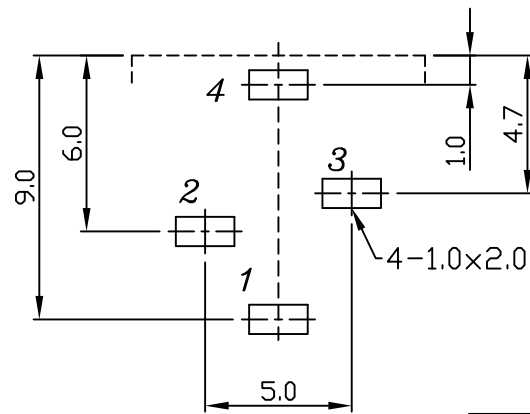
(BOTTOM VIEW) P.C.B. LAYOUT(±0.1)
