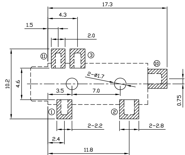
RECOMMENDED PCB LAYOUT TOLERANCE:±0.05 (TOP VIEW)
